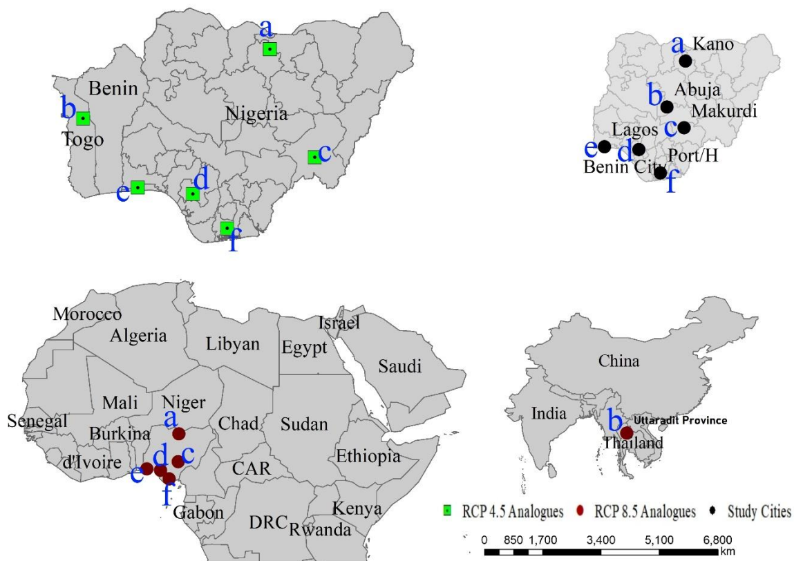
Figure 4.23a: Precipitation Analogues for 2050s. a. Kano b. Abuja c. Makurdi d. Benin e. Lagos f. Port Harcourt
