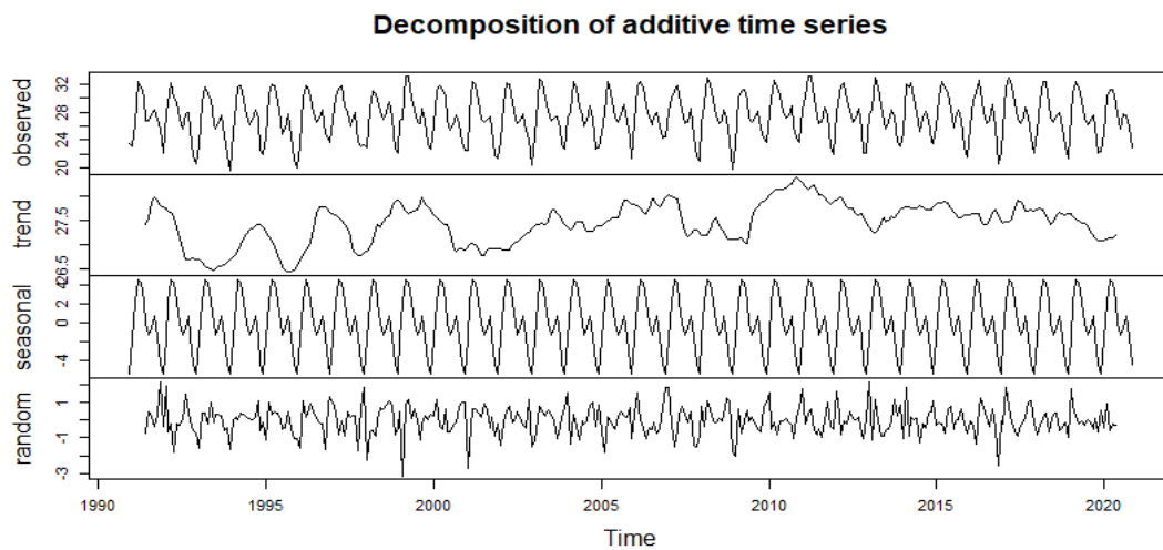
Figure 4.5: Kano Temperature Time Series
