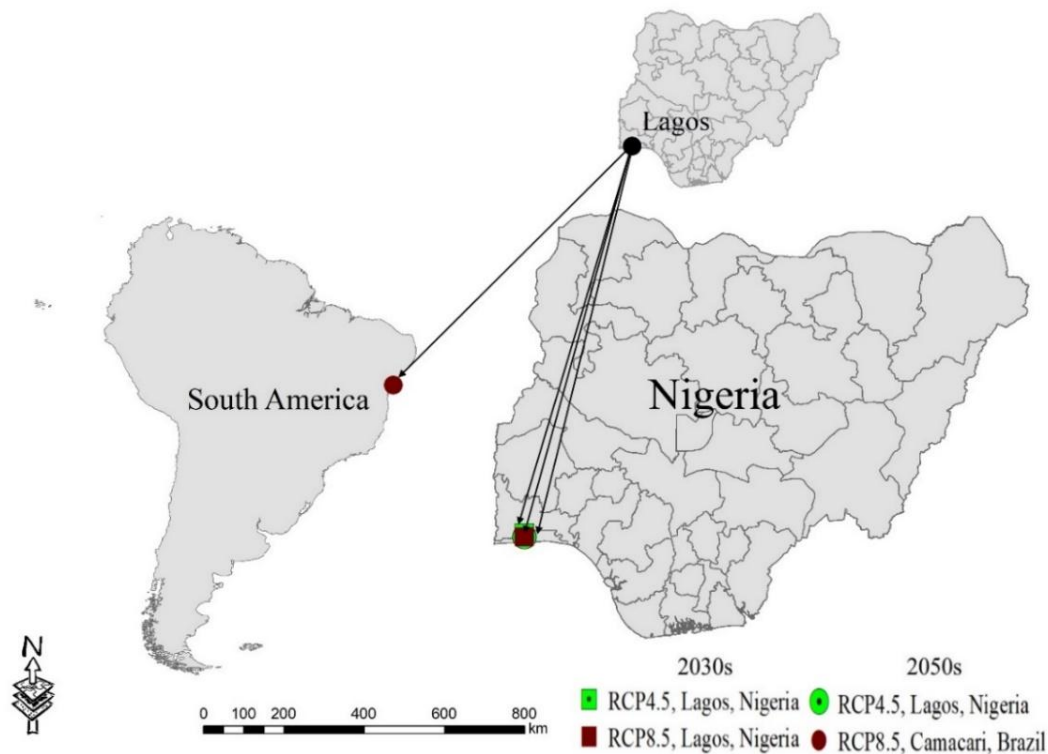
Figure 4.14: Climate of Lagos (2030s) and (2050s)
