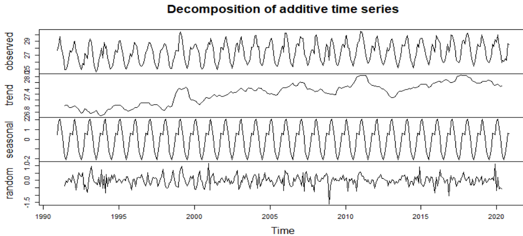
Figure 4.3: Lagos Temperature Time Series
