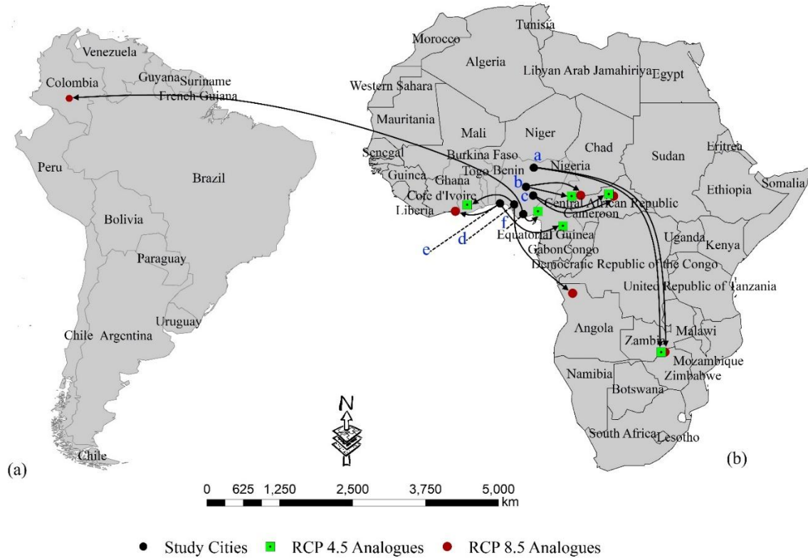
Figure 4.20a: Temperature analogues for the 2030s (RCP4.5 and 8.5 scenarios)
