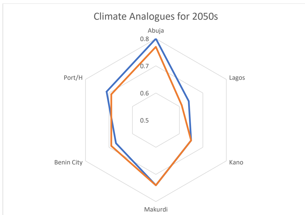
Figure 4.19a: Similarity Score of 2050s Climate Analogues
