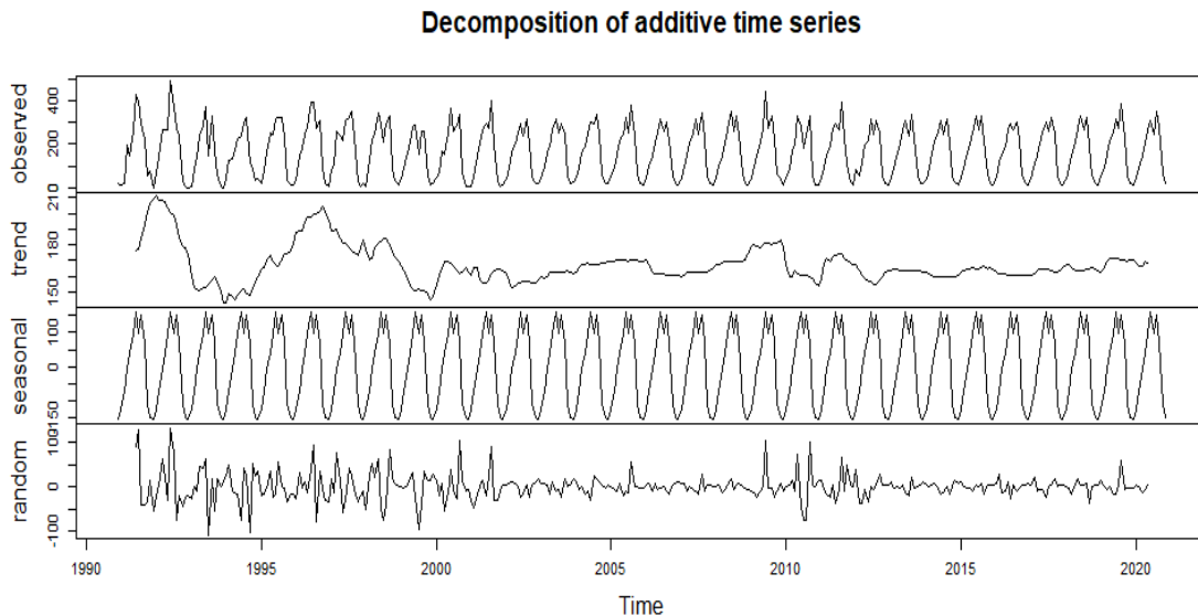
Figure 4.10: Benin Precipitation Time Series between 1990 and 2020
