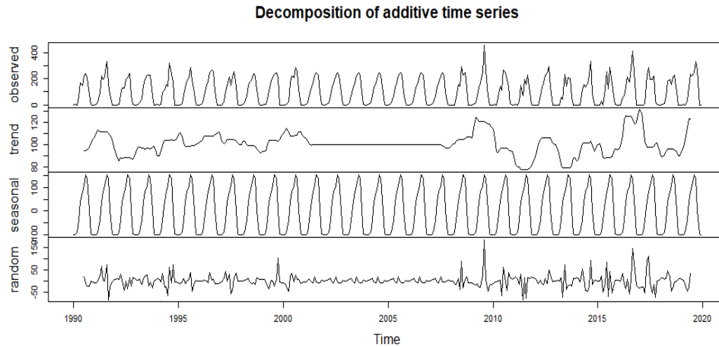
Figure 4.2: Abuja Precipitation Time Series
