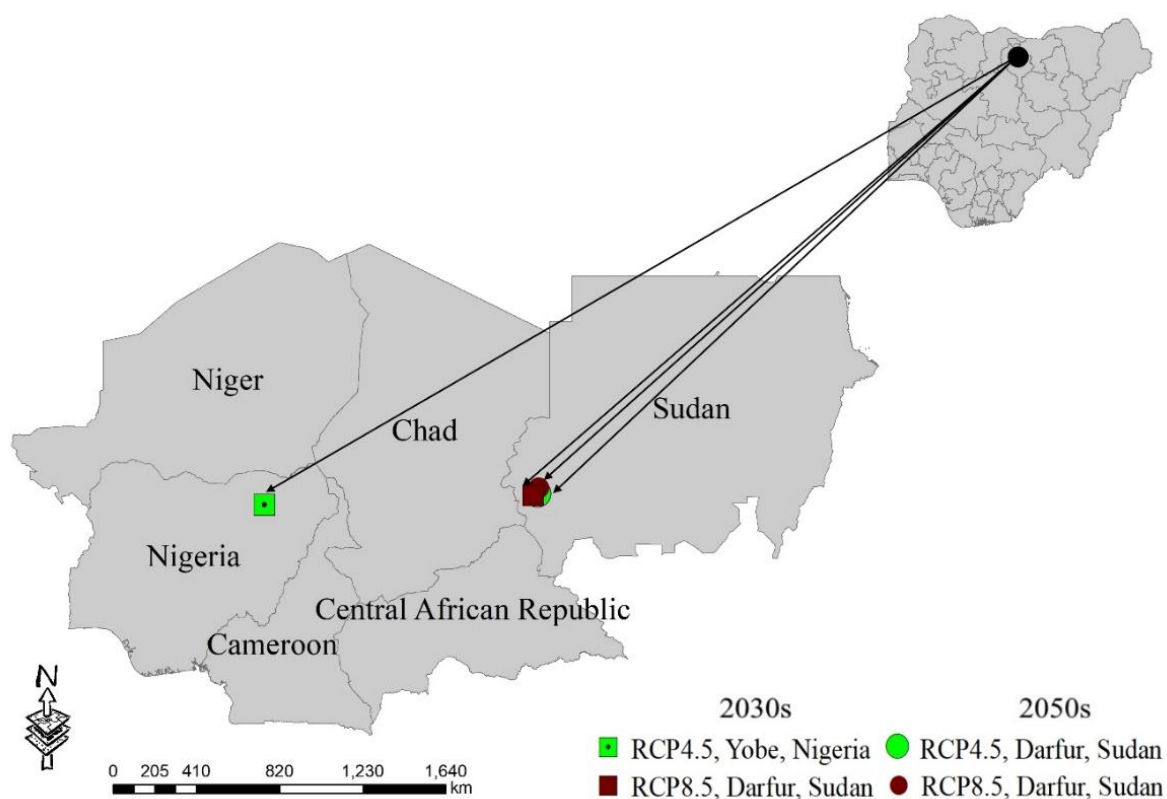
Figure 4.15: Climate of Kano (2030s) and (2050s).
