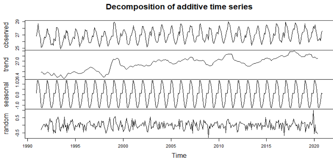
Figure 4.11: Port/Harcourt Temperature Time Series between 1990 and 2020
