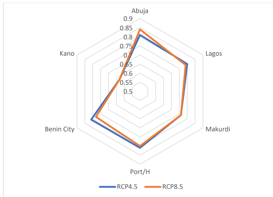
Figure 4.21b: 2050s Temperature Similarity for the Cities
