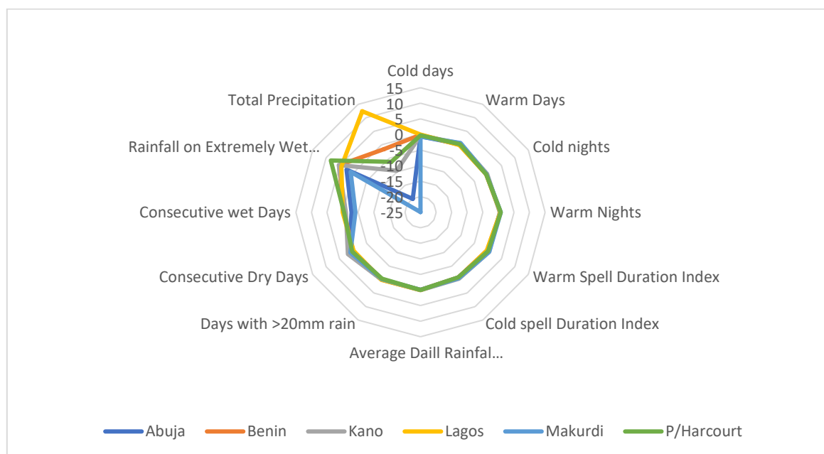
Figure 4.24: Magnitude of Change in Climate Indices for the Cities
