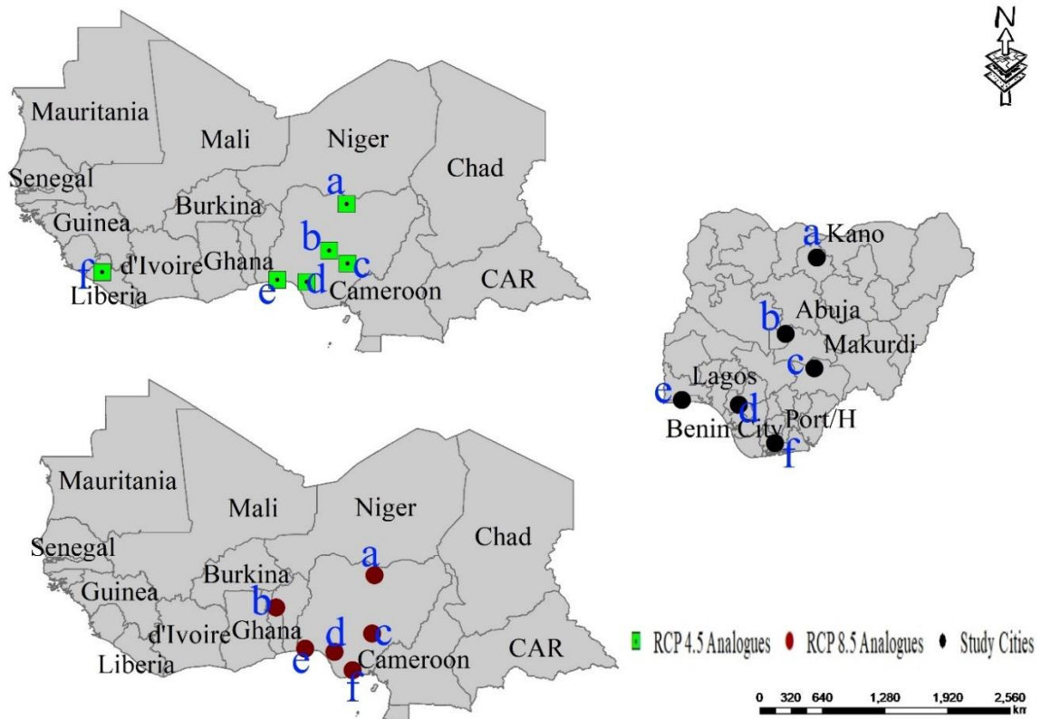
Figure 4.22a: Precipitation Analogues for 2030s a. Kano b. Abuja c. Makurdi d. Benin e. Lagos f. Port Harcourt
