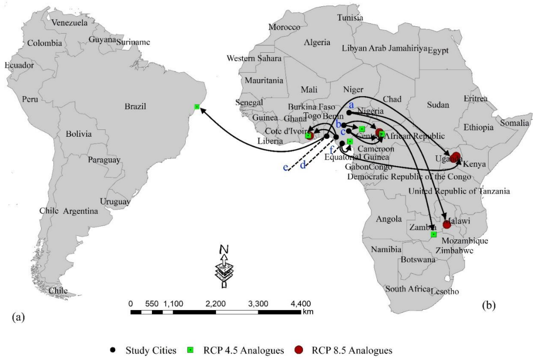
Figure 4.21a: Temperature analogues for the 2050s (RCP4.5 and 8.5 scenarios)
