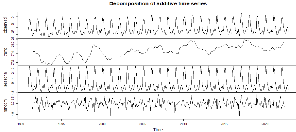
Figure 4.7: Makurdi Temperature Time Series between 1990 and 2020
