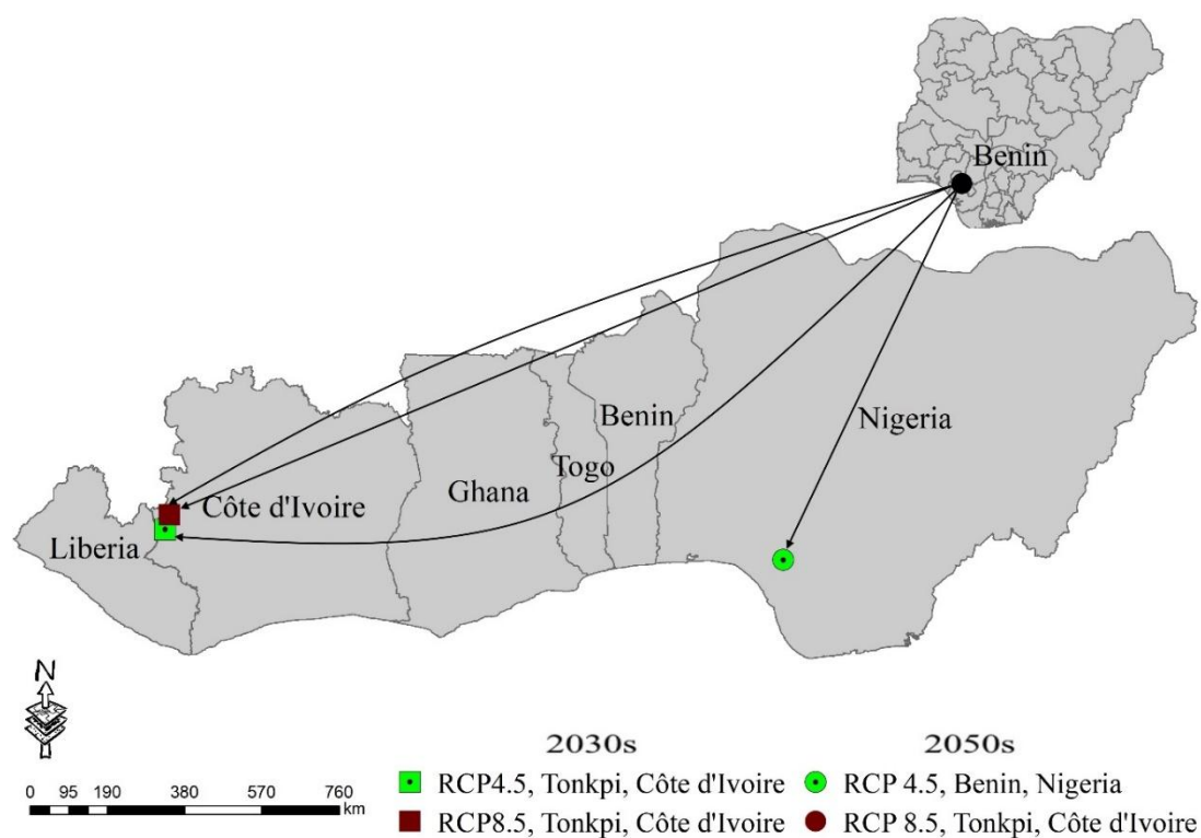
Figure 4.17: Future Climate of Benin (2030s) and (2050s)
