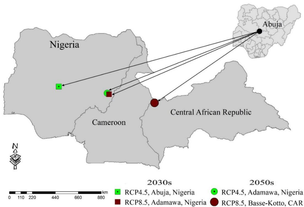
Figure 4.13: Climate of Abuja in (2030s) and (2050s)
