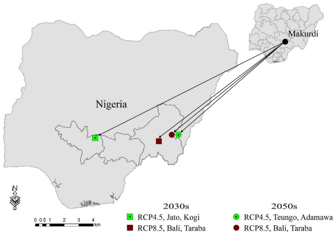
Figure 4.16: Climate of Makurdi (2030s) and (2050s)
