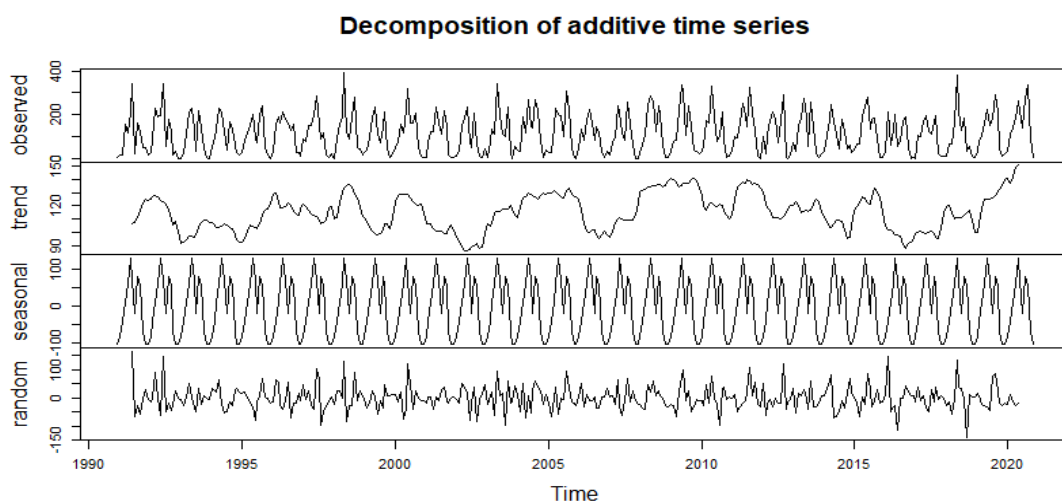
Figure 4.4: Lagos Precipitation Time Series
