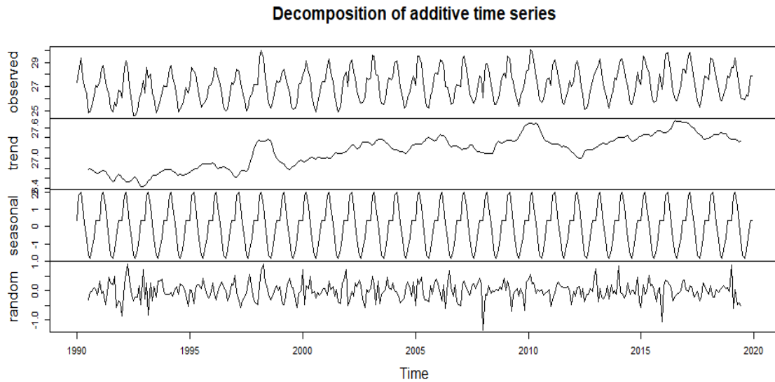
Figure 4.9: Benin Temperature Time Series between 1990 and 2020
