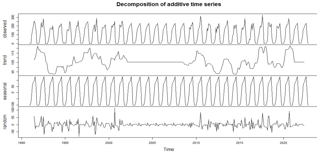
Figure 4.8: Makurdi Precipitation Time Series between 1990 and 2020
