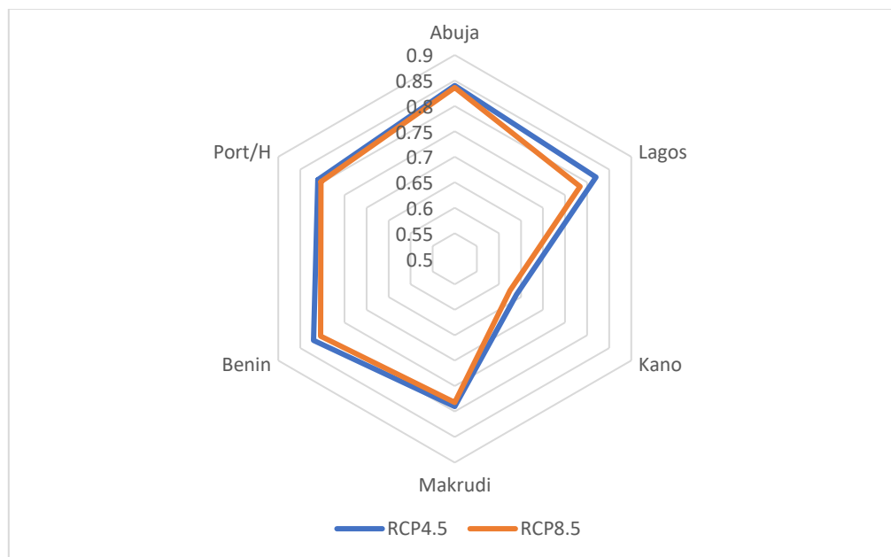
Figure 4.20b 2030s: Temperature Similarity for the Cities
