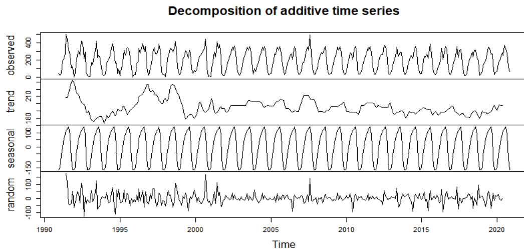
Future 4.12: P/Harcourt Precipitation Time Series.
