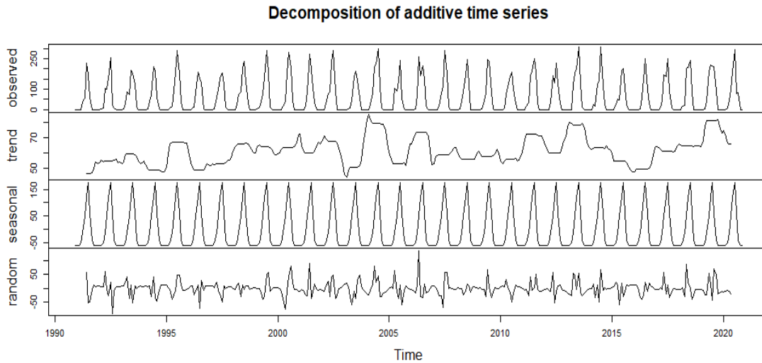
Figure 4.6: Kano Precipitation Time Series
