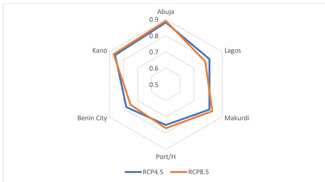
Figure 4.23b: 2050s Precipitation Similarity for the Cities
