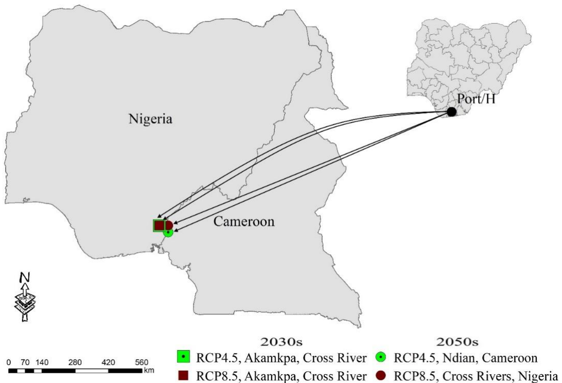
Figure 4.18: Future Climate of Port Harcourt (2030s) and (2050s)
