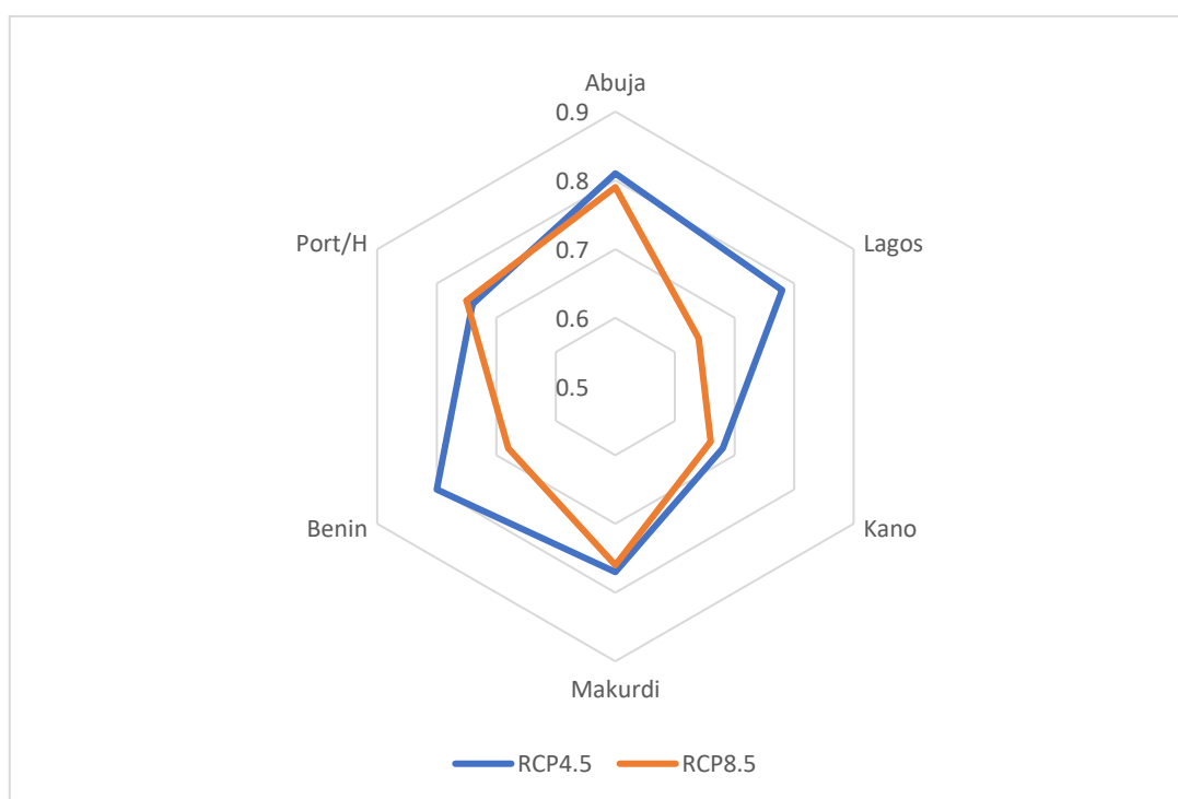
Figure 4.19b: Similarity Score of 2030s Climate Analogues
