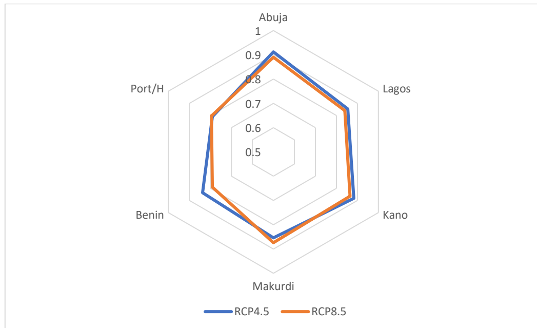
Figure 4.22b: 2030s Precipitation Similarity for the Cities
