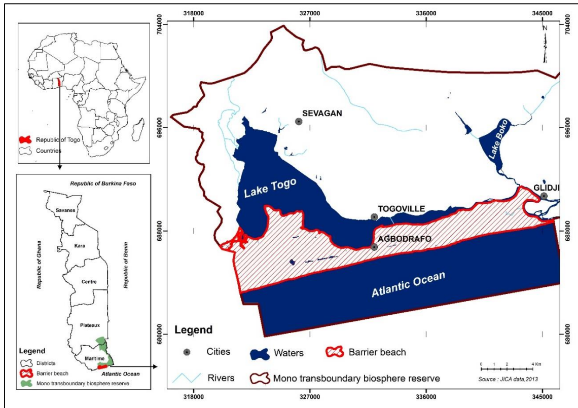
Figure. Segment from Aneho to Agbata located at the coastal facade of the reserve of mono biosphere
