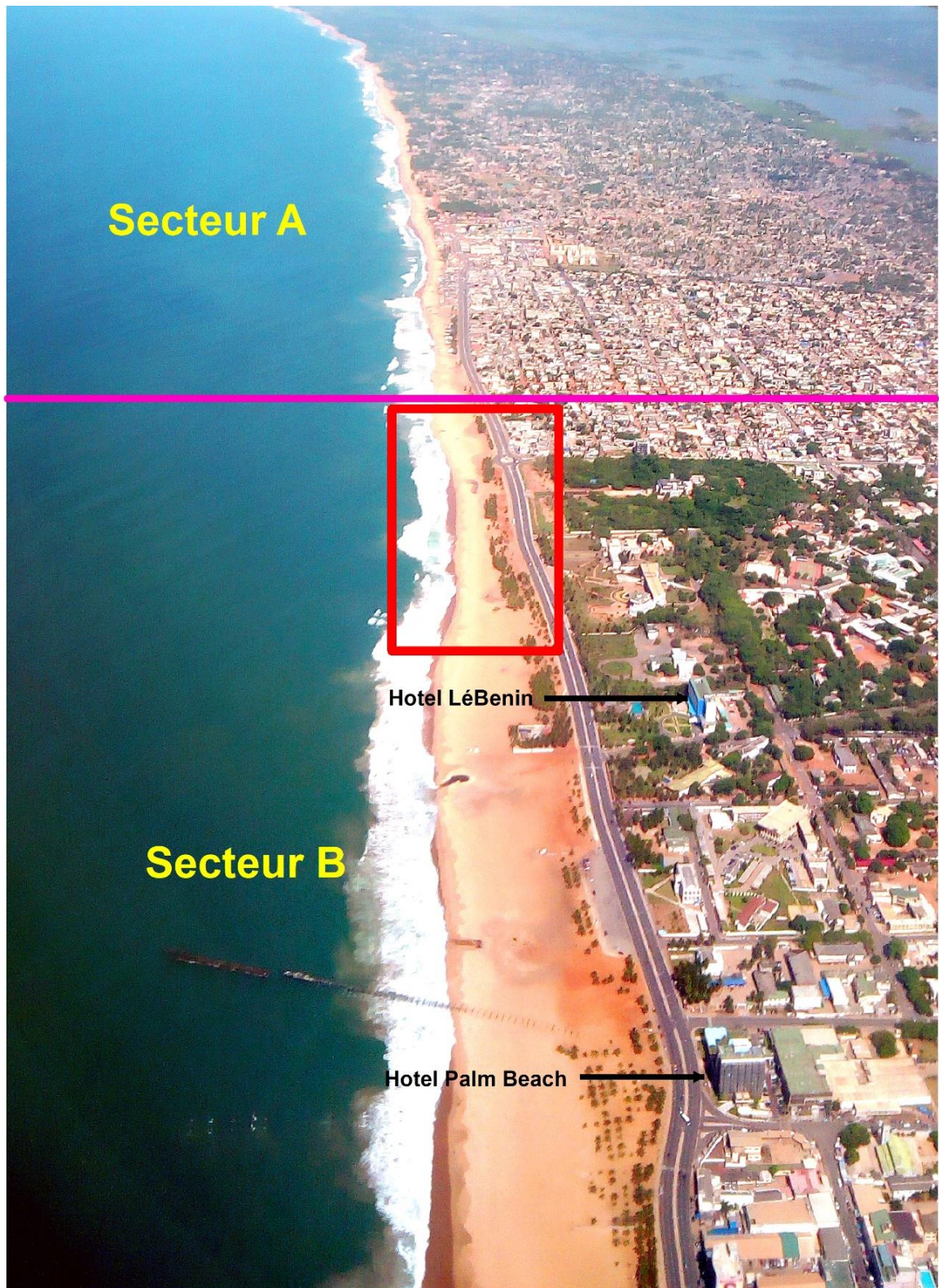
Plate II. Aerial photograph showing a sector of coastal erosion (A) and a sector of accretion (B). The erosion is very advanced and the sea is very close to the paved road in sector A. For sector B, an eroded portion is colored in red showing the sea nearby of the road.
