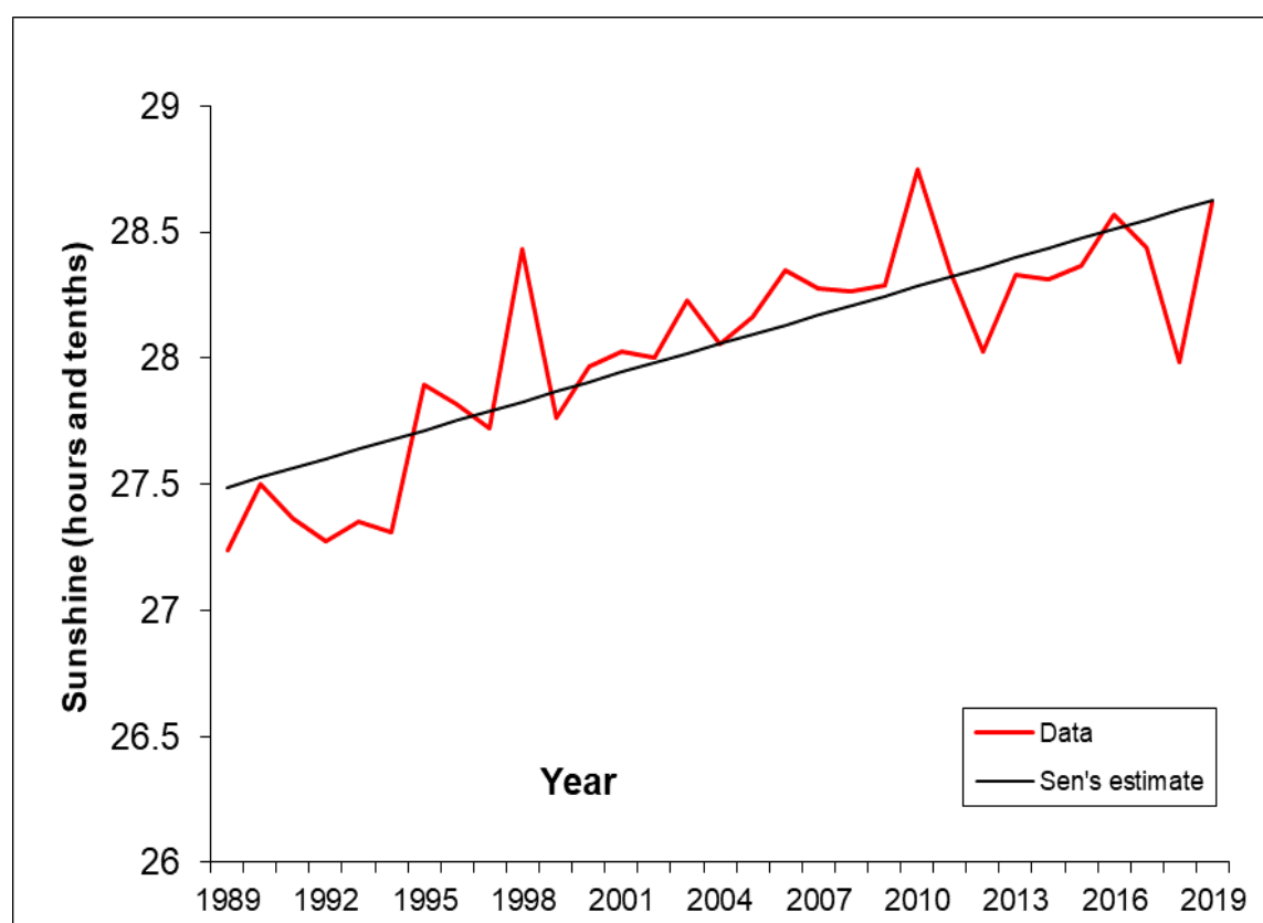
Figure 4.5. Annual trend of sunshine from 1989-2019 over Lomé city as shown by observation dataset.
