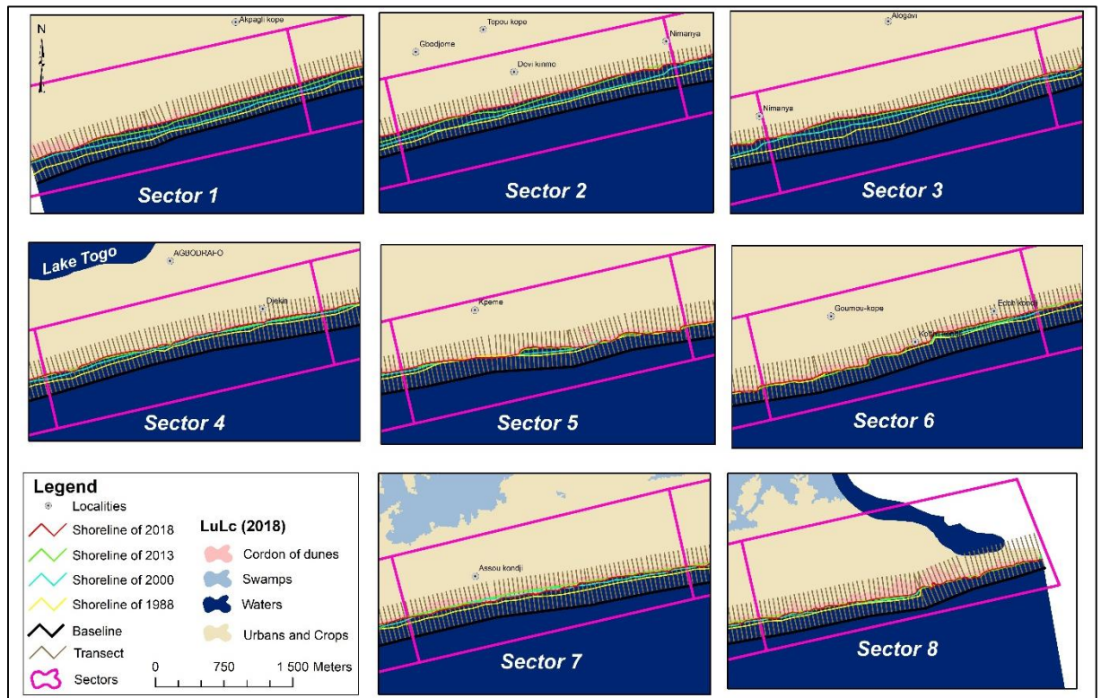
Figure 4.10. Map of shoreline change from 1988 to 2018. The red line indicates the position of shoreline in 2018, the green line the position in 2013, the blue line its position in 2000 and the yellow line the position of shoreline in 1988.
