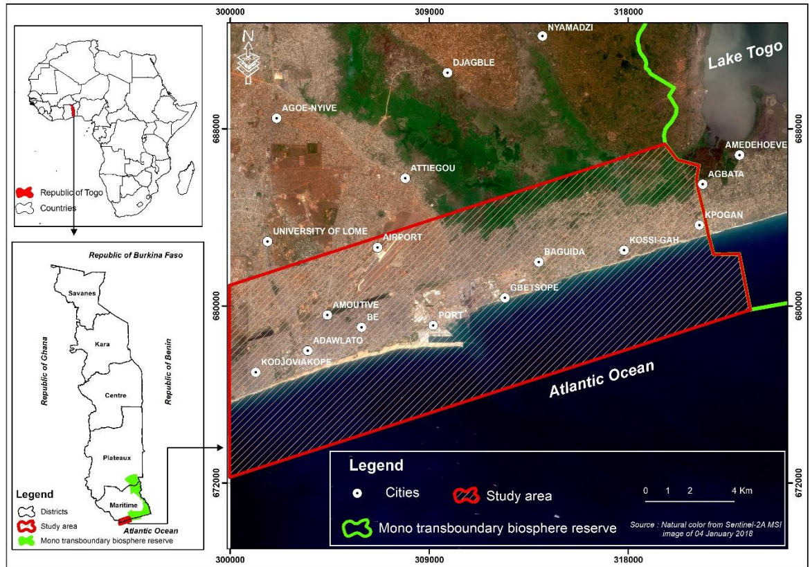
Figure. Segment from Agbata to Aflao located on the West part of coastal facade of the reserve of mono biosphere
