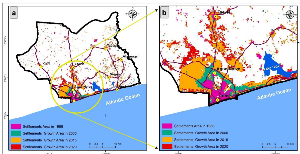
Figure 4.7. Spatio-temporal dynamics of settlement areas in lome. (a) Map showing settlements growth area; (b) Map showing the dynamics of settlements area in the city of Lome and surrounding.
