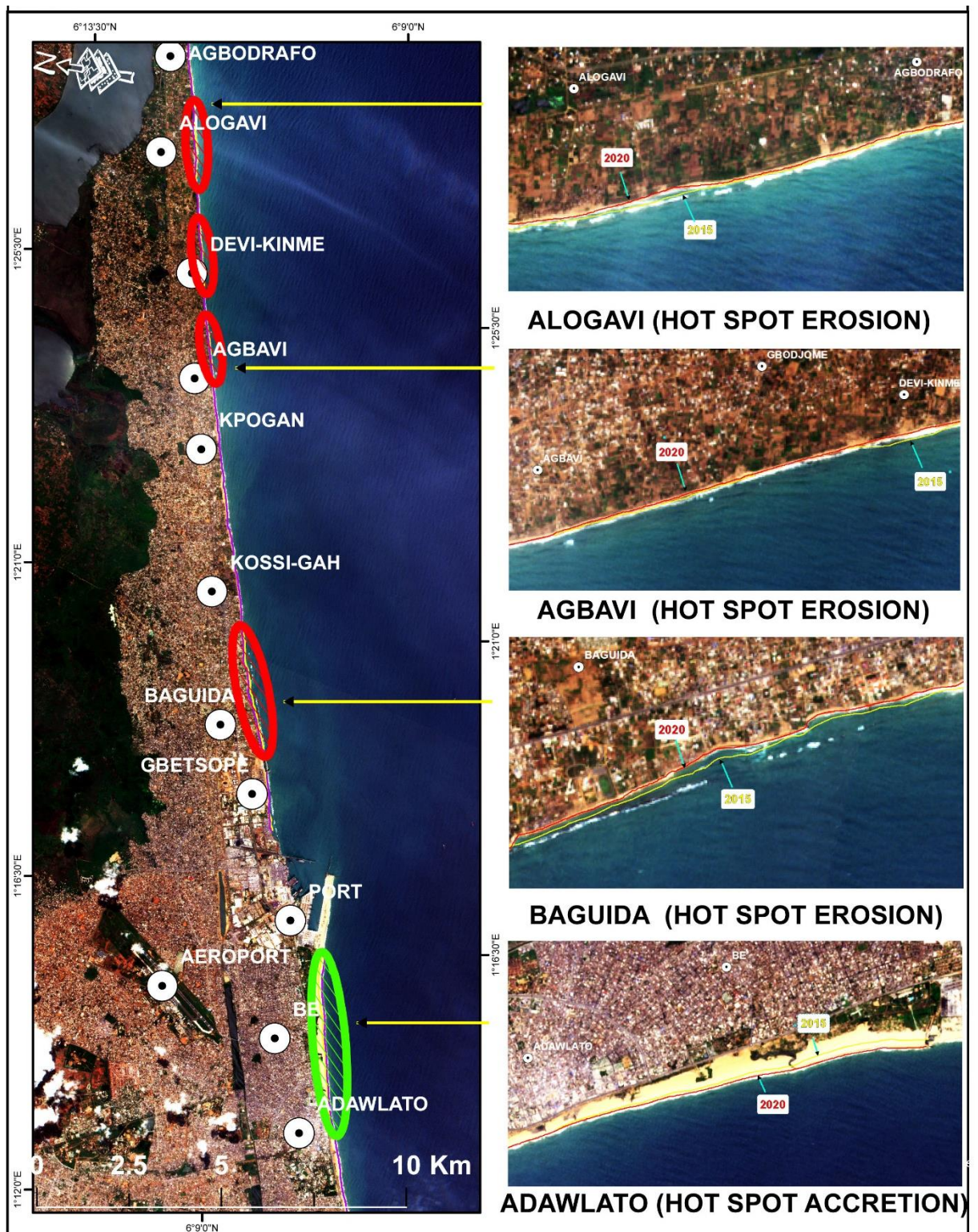
Figure 4.13. Map of Coastal Erosion HotSpots for the period 2015-2020
