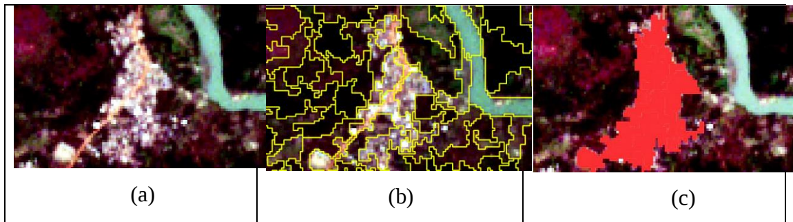
Figure 3.2. Overview of methodological approach for settlement area mapping. (a) Composite image of Sentinel-2 showing Settlements area; (b) Image segmented; (c) Settlements area classified.
