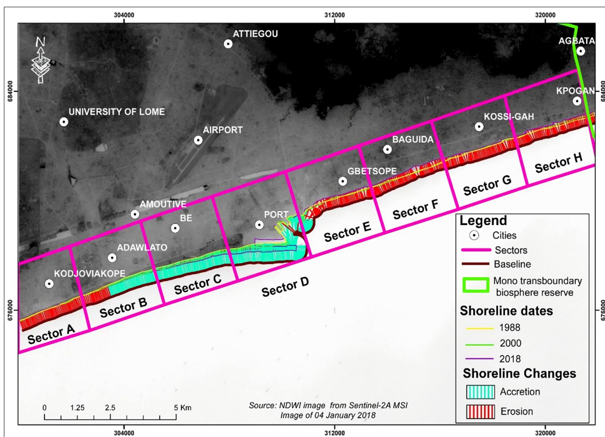
Figure 4.12. Evolution of the coastline on the Agbata-Aflao segment from 1988 to 2018
