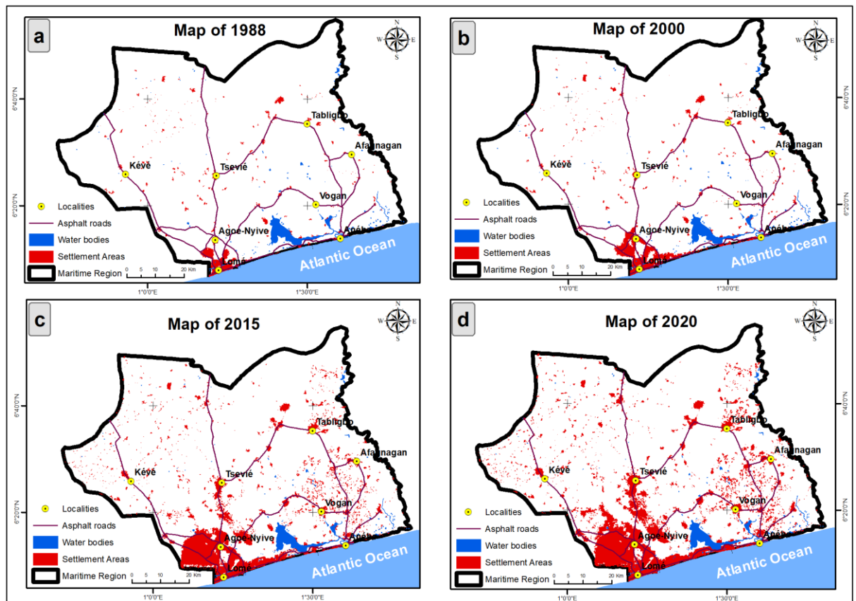
Figure 4.6. Spatio-temporal trend of settlements areas during the period 1988-2020. Maps of settlement areas in the following years (a) 1988; (b) 2000; (c) 2015; (d) 2020.
