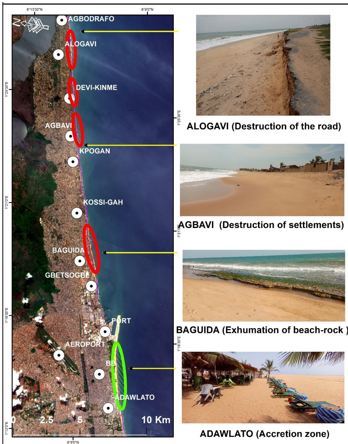
Figure 4.14. Illustration of Coastal Erosion HotSpots for the period 2015-2020
