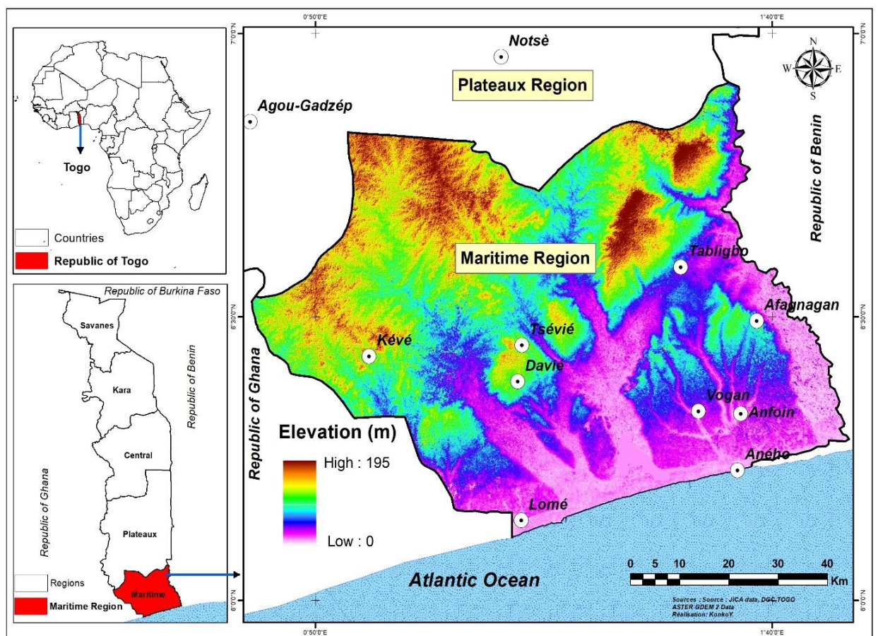
Figure 1.1. Area of study showing the Maritime region with digital elevation model in Togo
