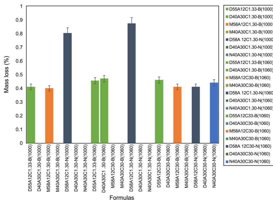
Figure 13. Mass lost by the different ceramic balls during heat treatment.
