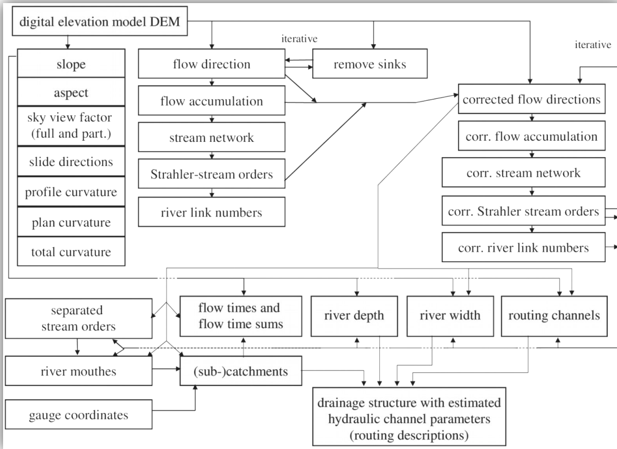
Figure 3.9: Topographic analysis of a digital elevation model by TANALYS (Schulla, 2012)
