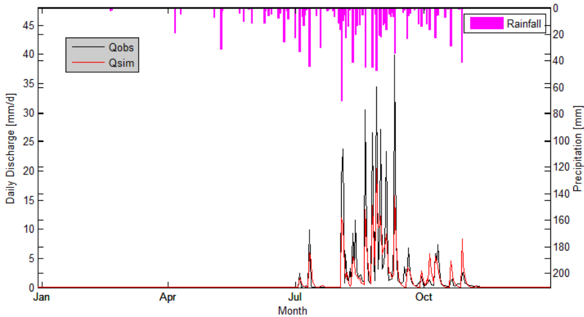
Figure 8.4: Observed vs simulated streamflow or discharge for the validation year (2015).
