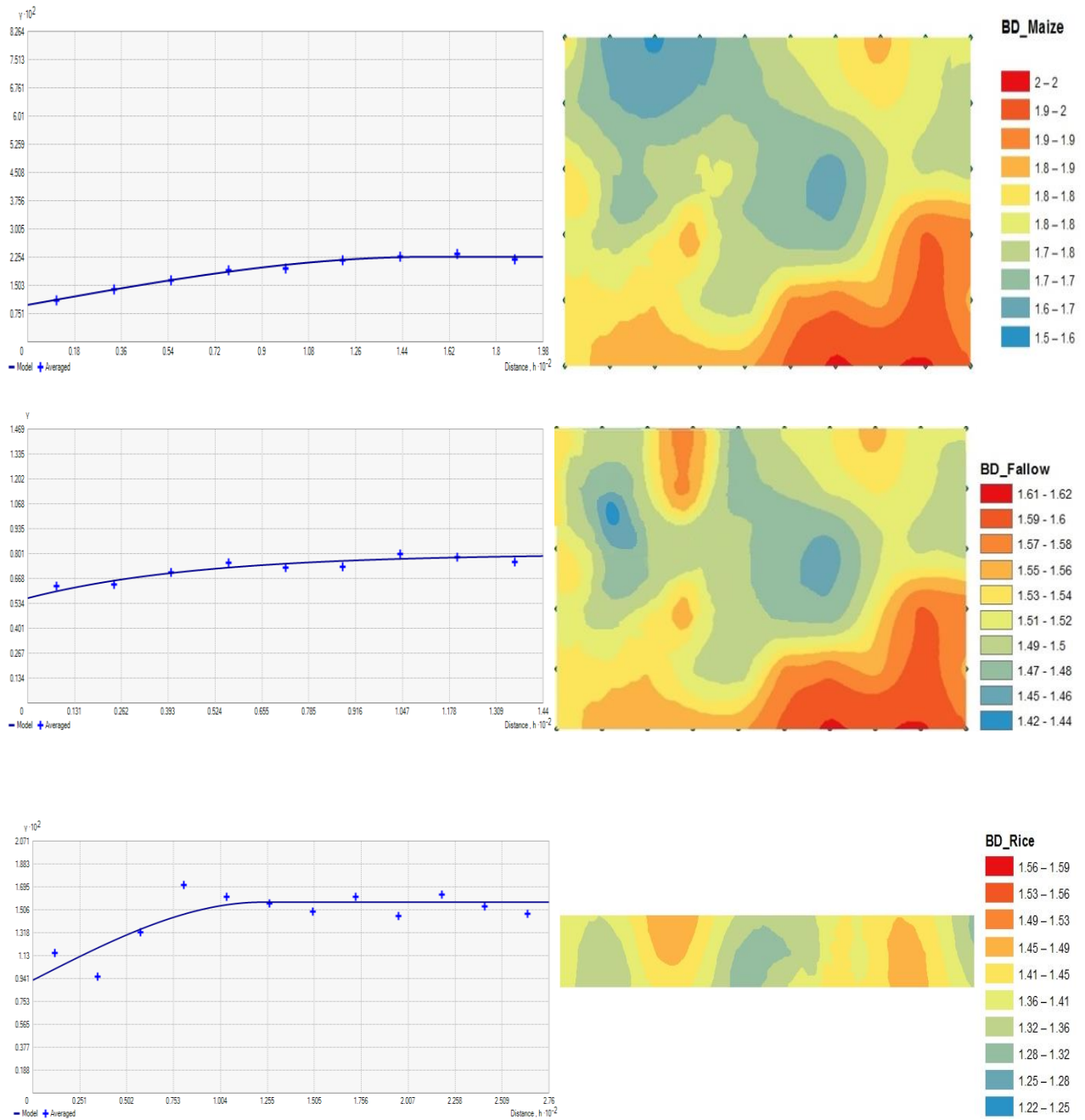
Figure 5.6: Variogram and mapping of bulk density (BD) under different land use.
