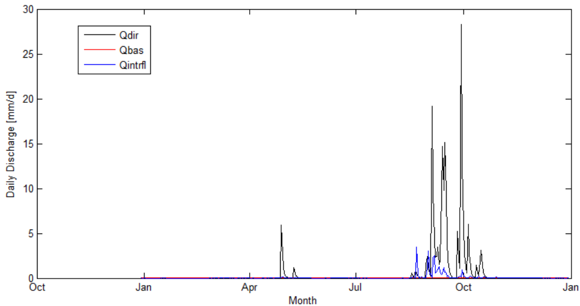
Figure 8.6: Hydrograph showing streamflow or discharge components for the calibration year (2014).
