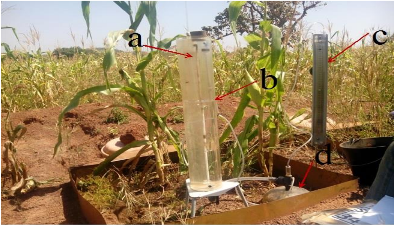
Figure 3.4: Set-up of hood infiltrometer during the field measurement in Koupendri catchment, a = bubble tower, b = water level reservoir, c = u-tube manometer, d = constant water level hood.
