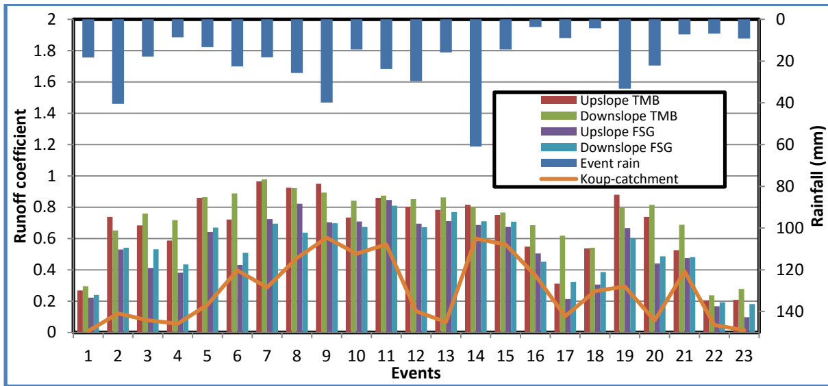
Figure 7.2: Runoff coefficient at the microplot and the catchment scale.
