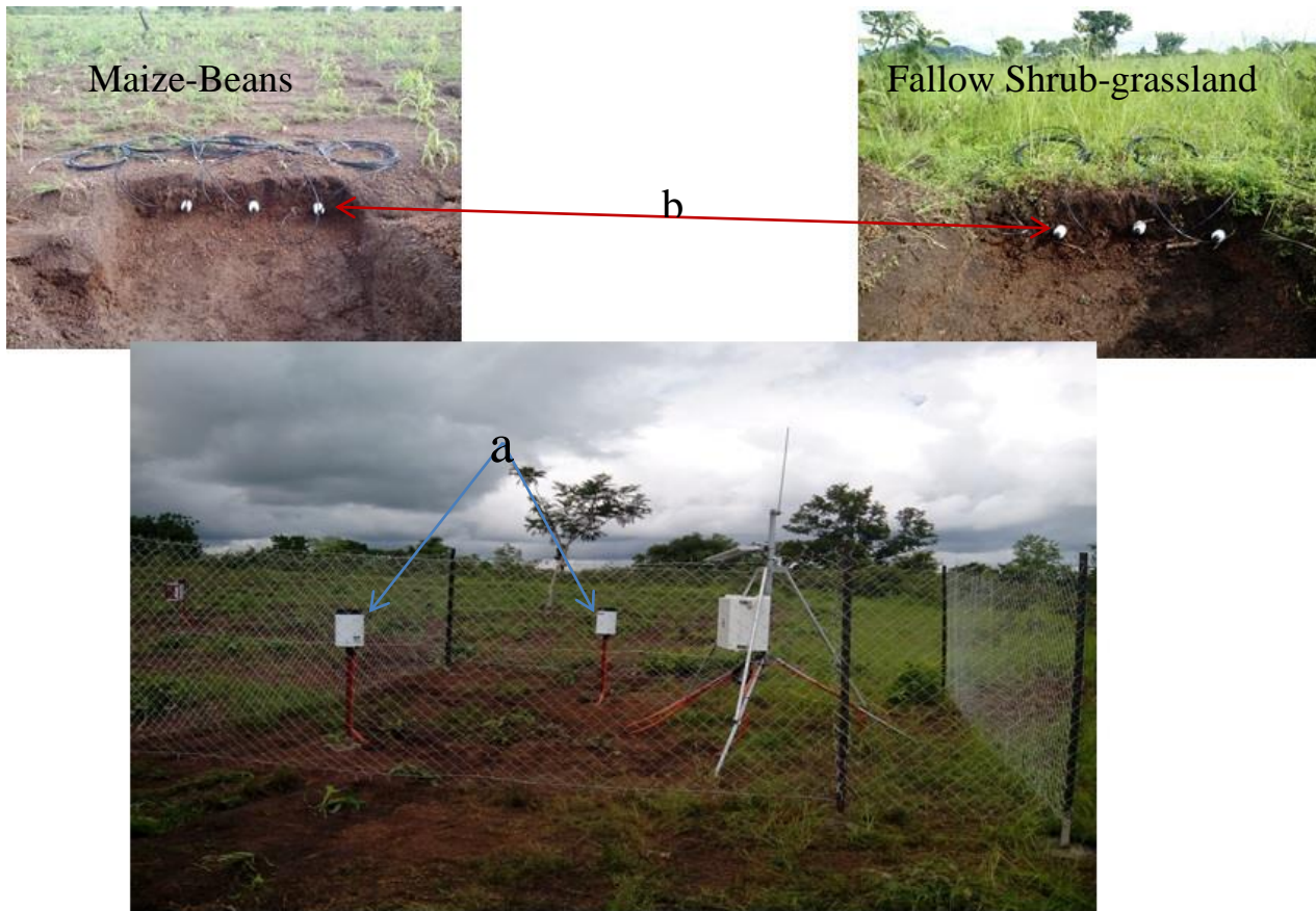
Figure 3.5: Installation of soil moisture sensors and raingauge at the soil-moisture station at Wanteou in Koupendri catchment; (a) Tipping bucket raingauge (b) soil moisture sensors.
