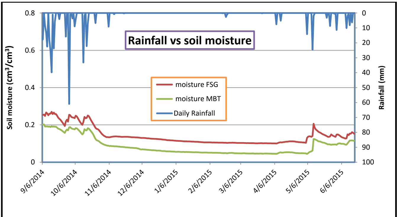
Figure 6.2: Temporal variability of rainfall and soil moisture dynamics under different land use at daily timescale.
