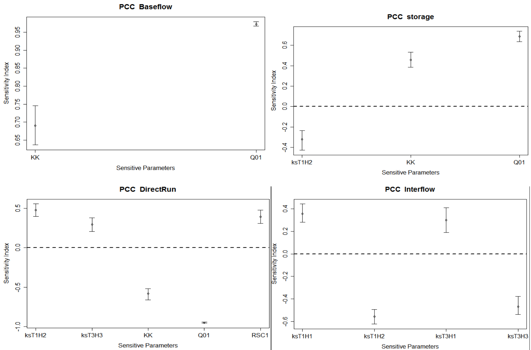
Figure 8.1: Sensitivity analysis results showing the sensitivity indices for the most sensitive parameters for directflow, interflow, baseflow and storage for WaSiM simulation at Koupendri catchment.
