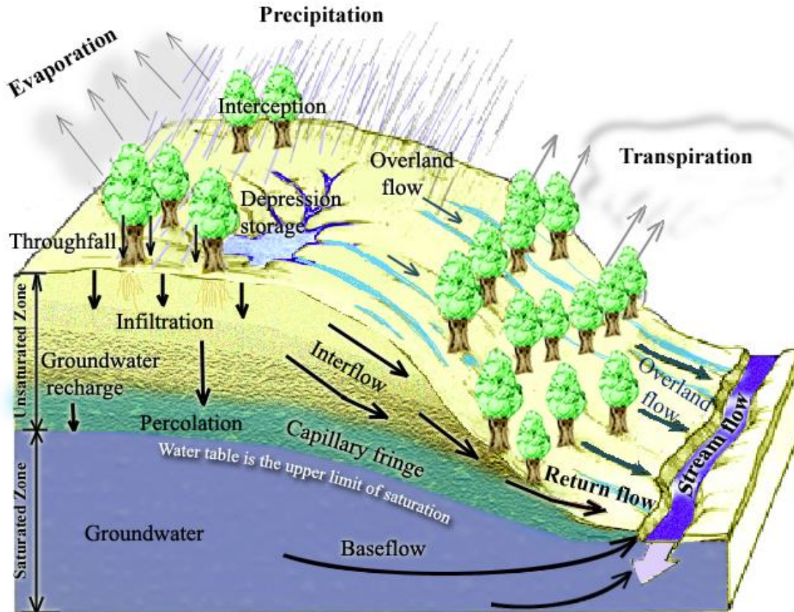
Figure 1.1: Physical Processes involved in Runoff Generation (Tarboton, D.G., 2003)
