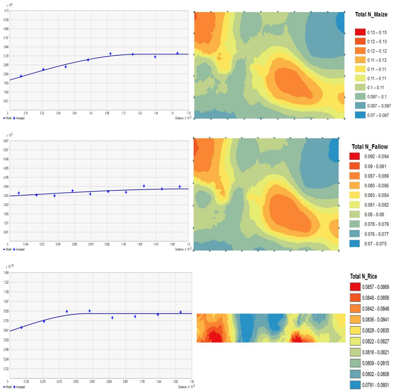
Figure 5.3: Variogram and mapping of total nitrogen (Total N) under different land use.
