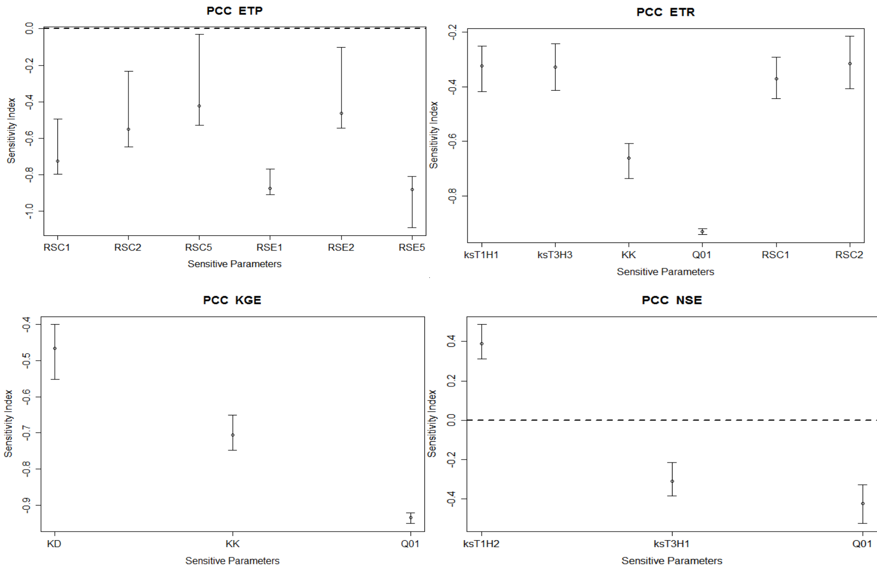
Figure 8.2: Sensitivity analysis results showing the sensitivity indices for the most sensitive parameters for ETpot, ETR, KGE and NSE for WaSiM simulation at Koupndri catchment
