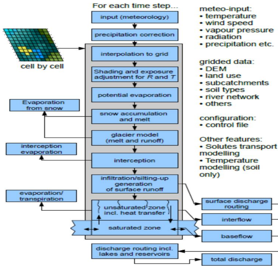
Fig. 3.8: Structure of the WaSiM model (Schulla, 2012)
