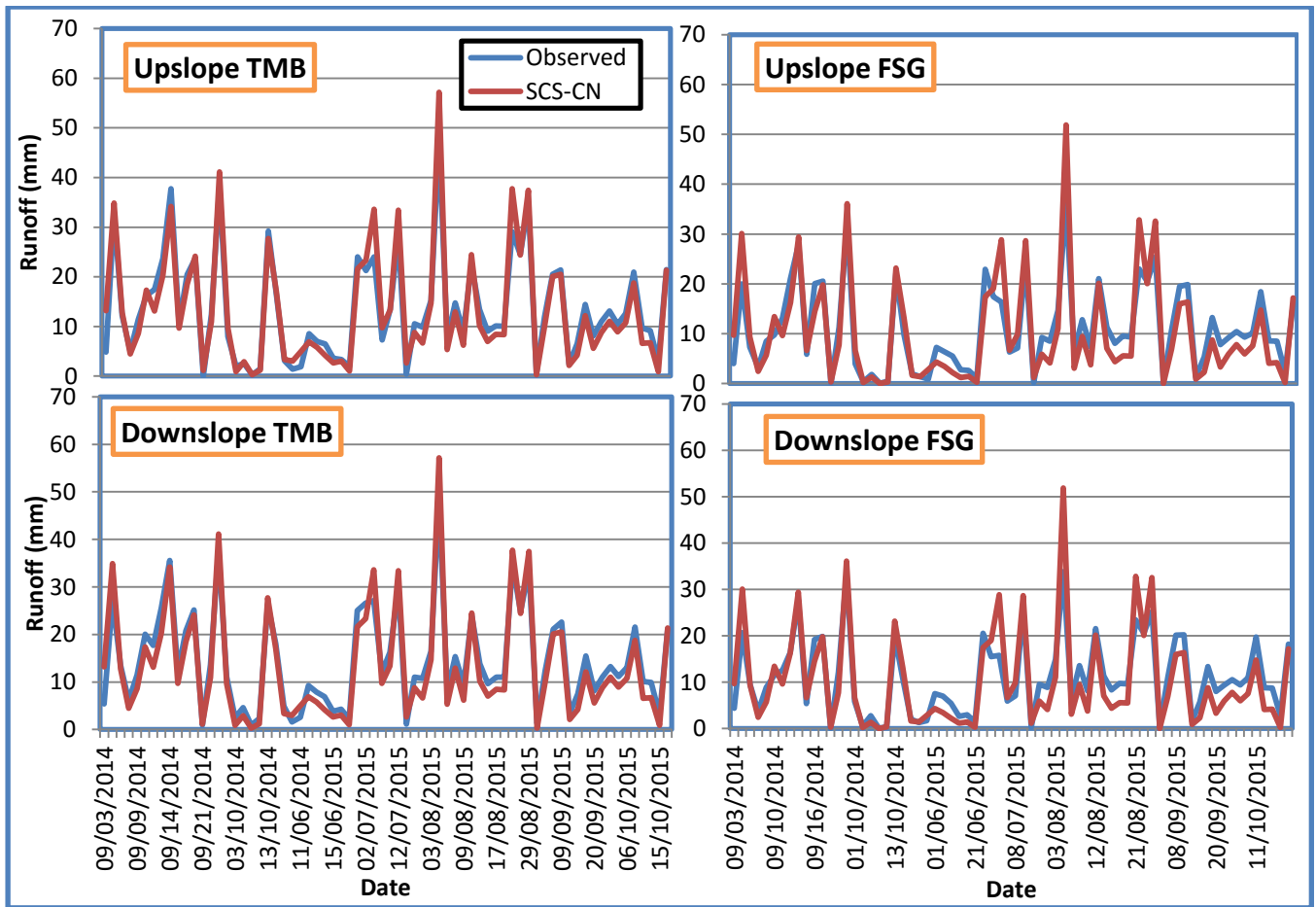
Figure 7.1: Observed and simulated runoff using NRCS-CN method for year 2014 and 2015.
