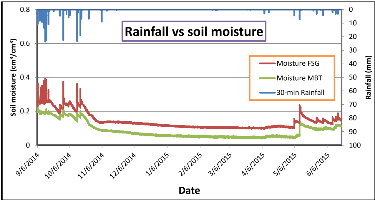
Figure 6.1: Temporal variability of rainfall and soil moisture dynamics under different land use at 30-minutes timescale.
