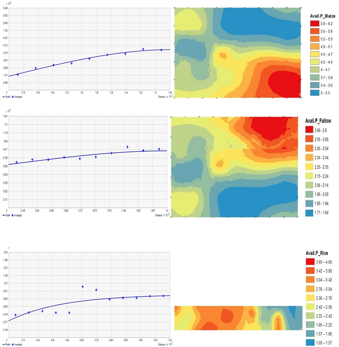
Figure 5.4: Variogram and mapping of available phosphorus (Avail.P) under different land use.
