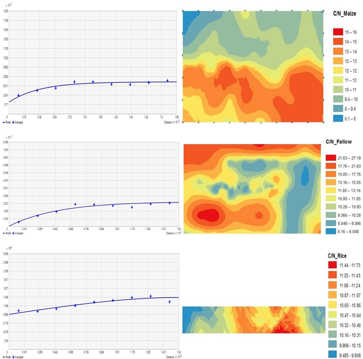
Figure 5.2: Variogram and mapping of carbon-nitrogen ratio (C:N) under different land use
