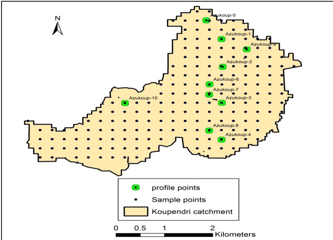
Figure 3.2: Map of the Koupendri catchment showing auger sampling and profile points
