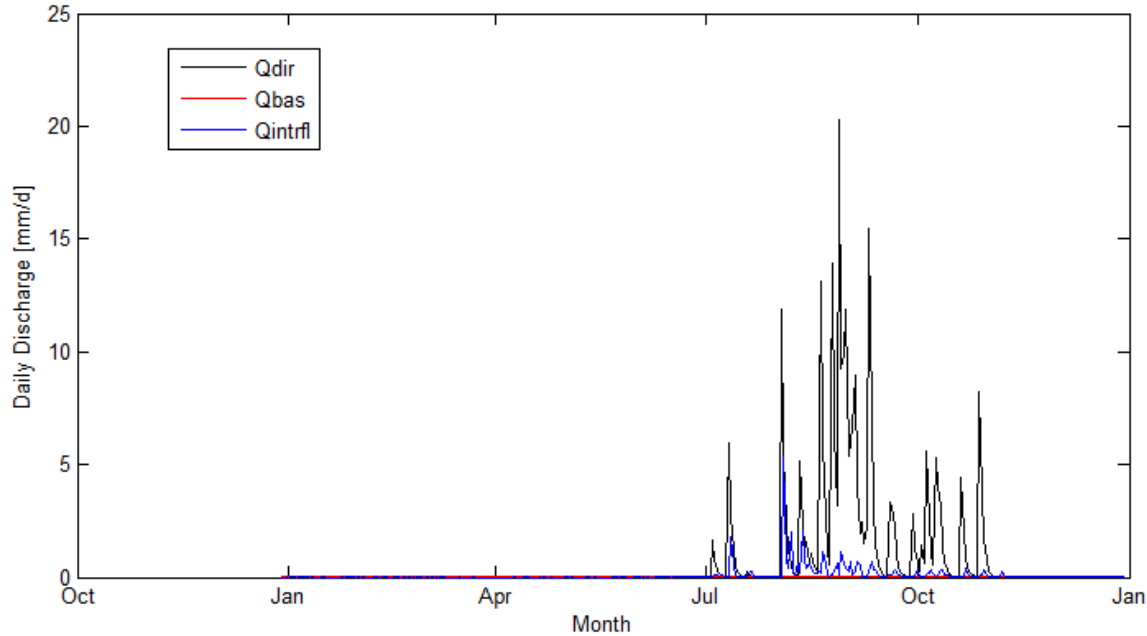
Figure 8.7: Hydrograph showing streamflow or discharge components for the validation year (2015).
