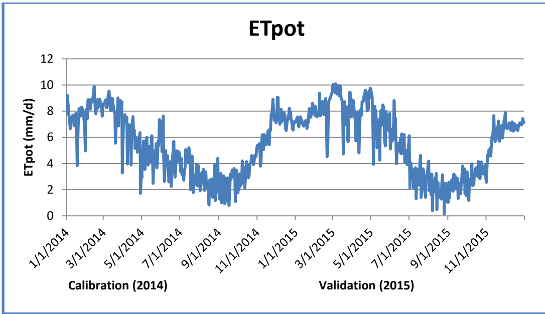
Figure 8.5: Daily ETpot of Koupendri catchment for the calibration and the validation year.
