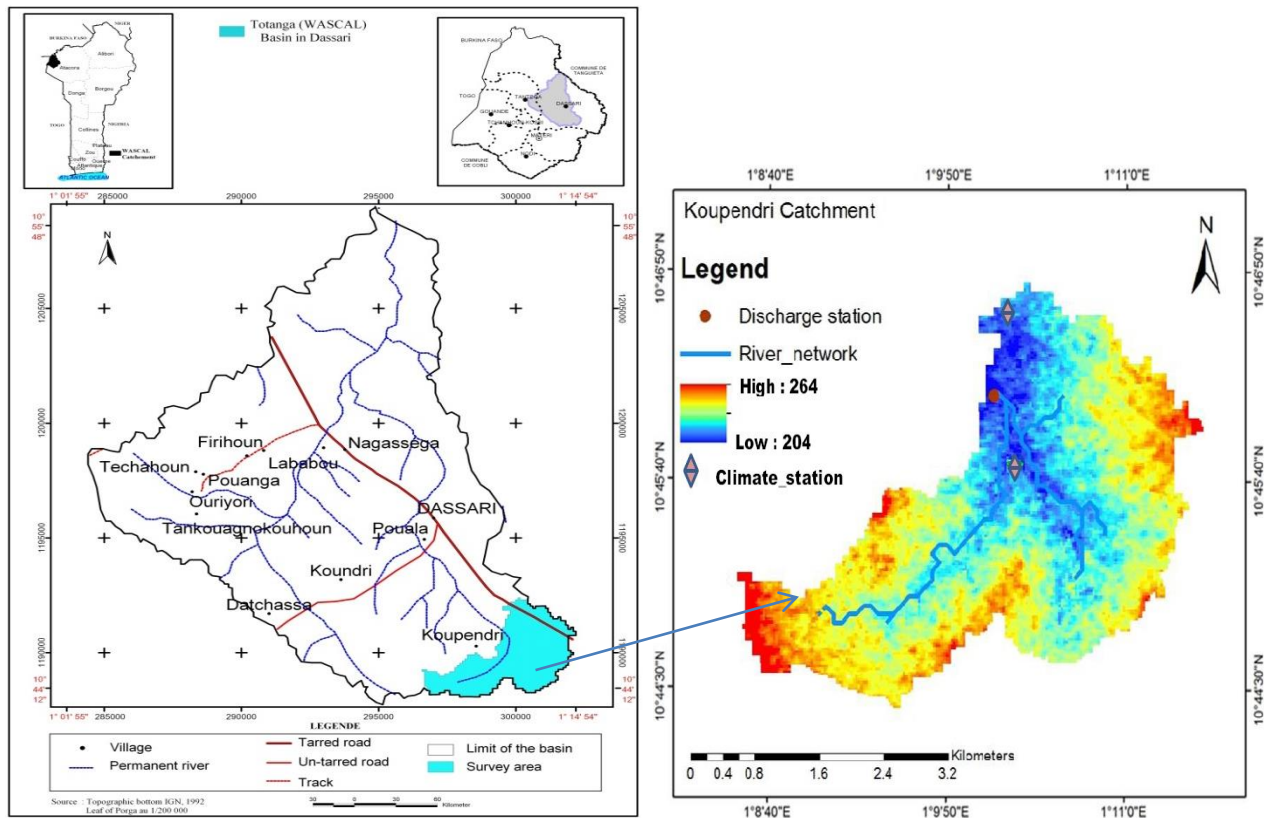
Figure 2.1: Location of Koupendri catchment in Benin.
