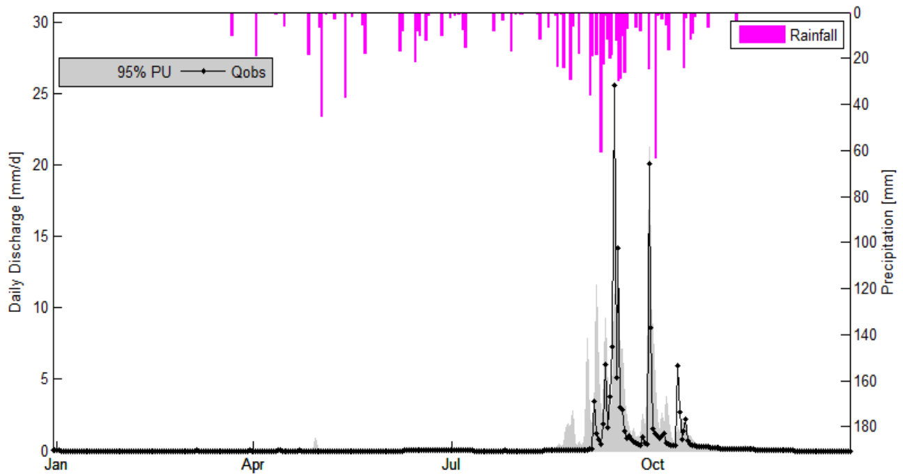
Figure 8.8: Model predictions uncertainty for the Koupendri catchment showing the measured daily discharge enclosed or bracketed by the 95 percent prediction uncertainties (95%PU).
