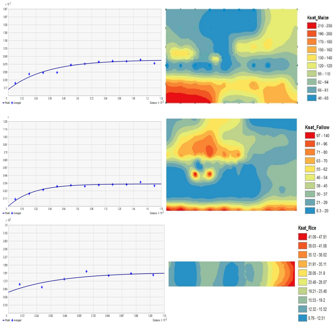
Figure 5.5: Variogram and mapping of saturated hydraulic conductivity under different land use
