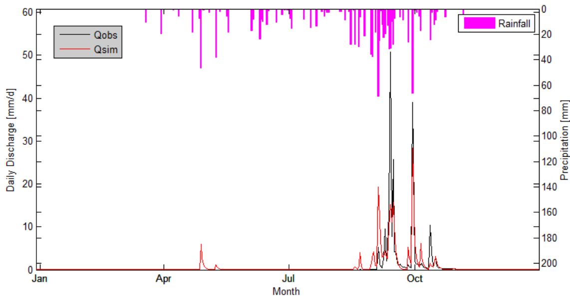
Figure 8.3: Observed vs simulated streamflow or discharge for the calibration year (2014).
