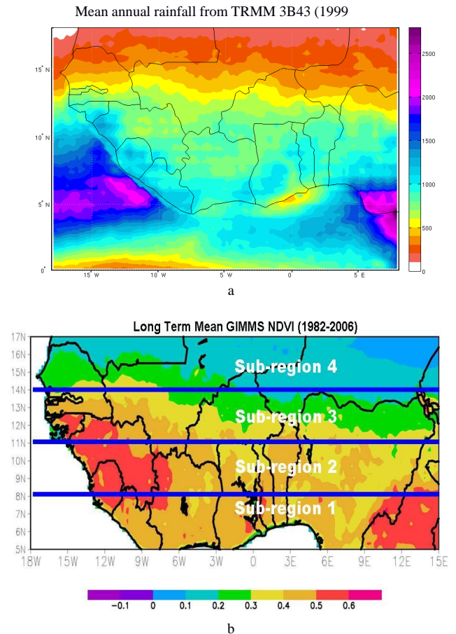
Figure 1. (a) Annual accumulated rainfall based on TRMM 3B43 data (1999–2006) and (b) mean normalized difference vegetation index (NDVI) over the regions. The boxes showing the subdivisions were made according to the climate division by Nicholson (2001).
